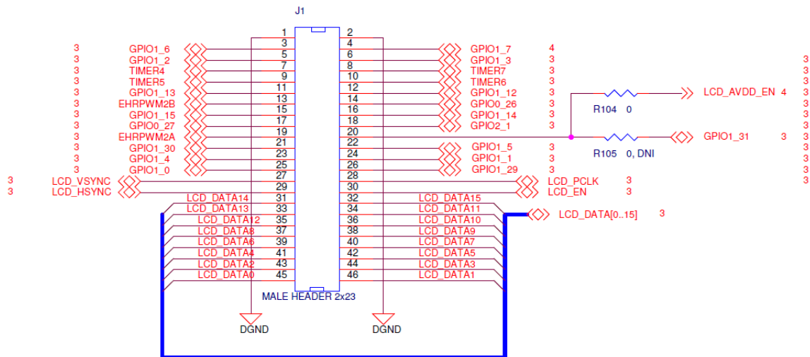
Figure 5. LCD Signals at expansion connector J1
