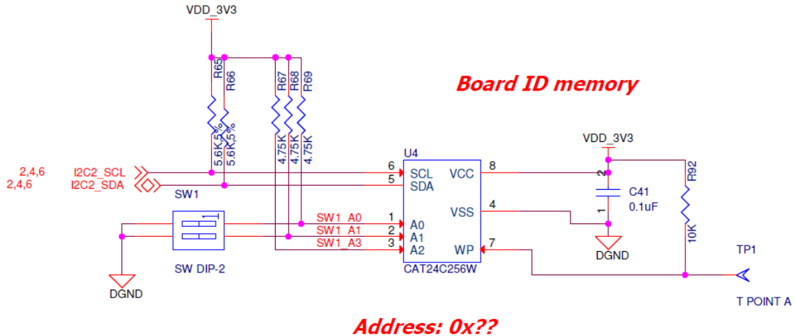
Figure 9. BeagleBone LCD7 Cape EEPROM
